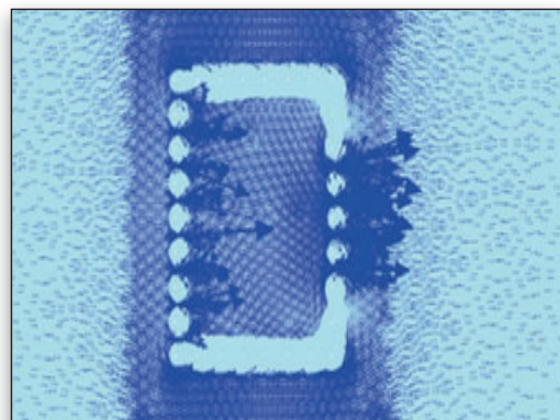
Figure 2: Water flow around freezing pipes.
